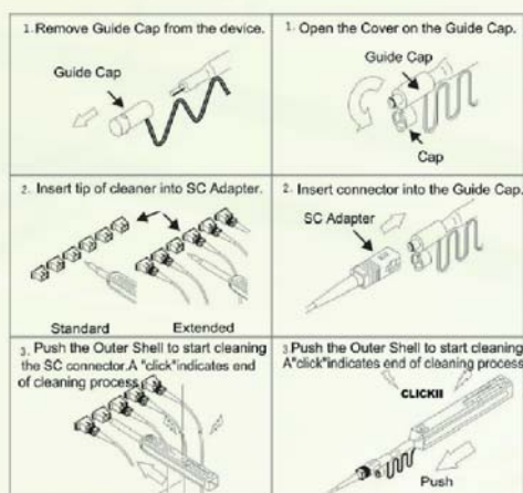
FC/SC/ST Application
