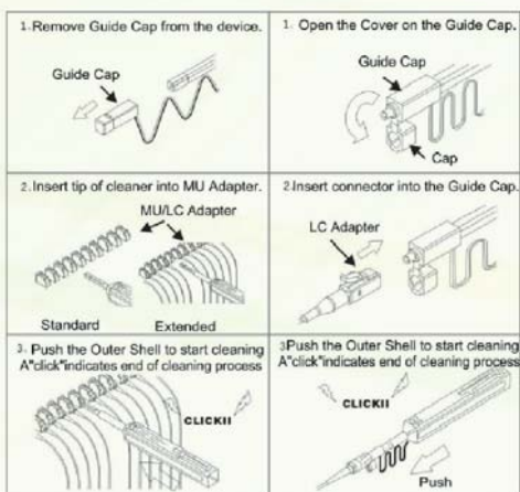
MU/LC Application
