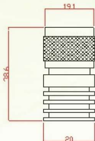
25W/30W RF Dummy Load
