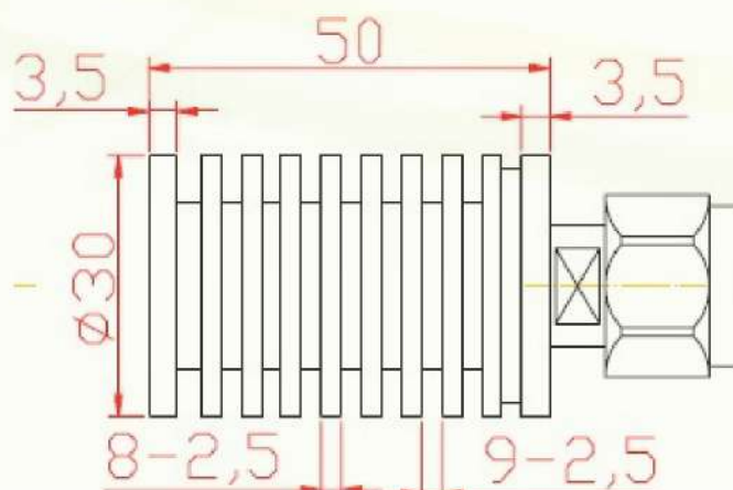
50W RF Dummy Load
