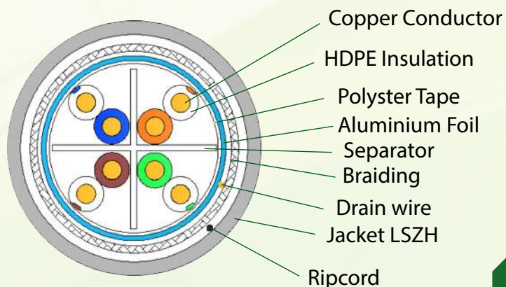
Electrical Characteristics ( CAT 6 - AWG 24 )
